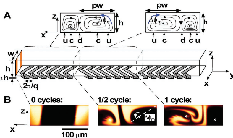
Fig. 2. Staggered herringbone mixer (SHM). (A) Schematic diagram of one-and-a-half cycles of the SHM. A mixing cycle is composed of two sequential regions of ridges; the direction of asymmetry of the herringbones switches with respect to the centerline of the channel from one region to the next. The streamlines of the flow in the cross section are shown schematically above the channel. The angle, \Delta\phi_m , is the average angular displacement of a volume of fluid along an outer streamline over one half cycle in the flow generated by the wide arms of the herringbones. The fraction of the width of the channel occupied by the wide arms of the herringbones is p . The horizontal positions of the centers of rotation, the upwellings, and the downwellings of the cellular flows are indicated by c , u , and d , respectively. (B) Confocal micrographs of vertical cross sections of a channel as in (A). Two streams of fluorescent solution were injected on either side of a stream of clear solution (29). The frames show the distribution of fluorescence upstream of the features, after one half cycle, and after one full cycle. The fingerlike structures at the end of the fluorescent filaments on the bottom left of the second two frames are due to the weak separation of streamlines that occurs in the rectangular grooves even at low Re . In this experiment, h = 77 \mu\text{m} , w = 200 \mu\text{m} , \alpha = 0.23 , q = 2\pi/100 \mu\text{m}^{-1} , p = 2/3 , and \theta = 45^\circ , and there were 10 ridges per half cycle. Re < 10^{-2} . \Delta\phi_m \sim 180^\circ .
